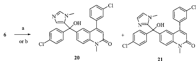
Scheme 4. a) 1. N -methylimidazole, n BuLi, ClSiEt 3 , THF, -78\text{ }^{\circ}\text{C} ; 2. n BuLi, -78\text{ }^{\circ}\text{C} , 20 (52%), 21 (4%); b) 1. N -methylimidazole, n -hexyllithium, ClSi( i Bu) 3 , THF, -78\text{ }^{\circ}\text{C} ; 2. n -hexyllithium, -78\text{ }^{\circ}\text{C} , 20 (75%), 21 (< 0.3%)
