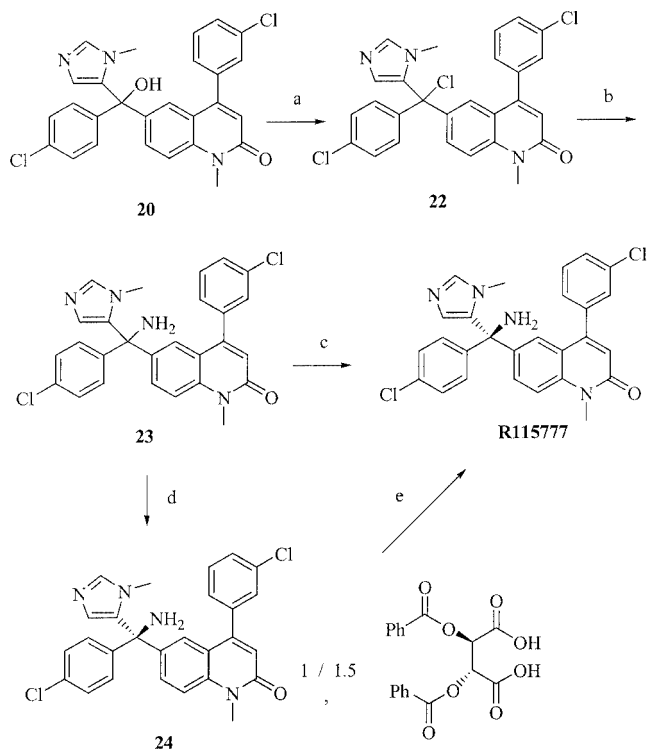
Scheme 5. a) SOCl 2 , 40\text{ }^{\circ}\text{C} or HCl, SOCl 2 , N,N -dimethylimidazolidinone, room temp.; b) NH 4 OH, THF, 80\text{ }^{\circ}\text{C} (65%) or NH 3 /MeOH, room temp. (70–75%); c) enantiomer separation by HPLC on chiral phase (32.5%); d) L-(–)-dibenzoyltartaric acid monohydrate, acetone, room temp. (37%); e) NH 4 OH, EtOH, 80\text{ }^{\circ}\text{C} (86%)
