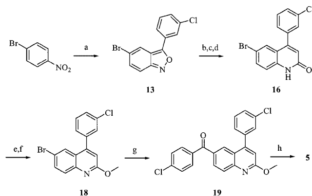
Scheme 3. a) (3-Cl-C_6H_4)CH_2CN , NaOH, MeOH, room temp., 16 h (35%); b) TiCl_3 , H_2O/THF , room temp., 16 h (85%); c) Ac_2O , toluene, 110 °C, 2 h; d) t BuOK (4 equiv.), DME, room temp., 16 h (81%); e) POCl_3 , 80 °C, 16 h; f) MeONa/MeOH, 60 °C, 16 h (86%); g) (4-Cl-C_6H_4)C(O)N(CH_3)OCH_3 , n BuLi, THF, -70 °C, 0.5 h (75%); h) HCl (6 N), MeOH, 60 °C, 72 h, (80%)
