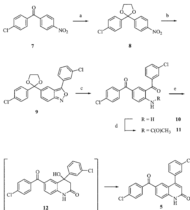
Scheme 2. a) Ethylene glycol, para -toluenesulfonic acid (PTSA), toluene, 110 °C, 24 h (98%); b) (3-Cl-C_6H_4)CH_2CN , NaOH, MeOH, 60 °C, 1 h (86%); c) TiCl_3 , H_2O/THF , room temp., 16 h; d) Ac_2O , toluene, 110 °C, 2 h; e) t BuOK (4 equiv.), DME, room temp., 3 h (87%)
