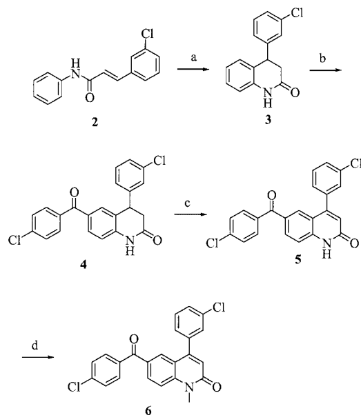
Scheme 1. a) Polyphosphoric acid (PPA), 100 °C, 16 h; b) 4-chlorobenzoic acid, 140 °C, 48 h (45%); c) Br_2 , C_6H_5Br , 160 °C, 16 h (93%); d) CH_3I , benzyltriethylammonium chloride (BTEAC), NaOH, THF, room temp., 16 h (75%)
